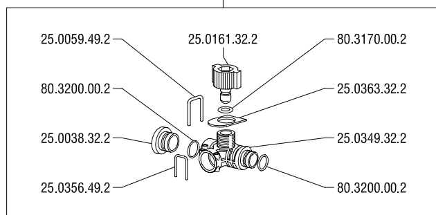
Intermediate by-pass kit
