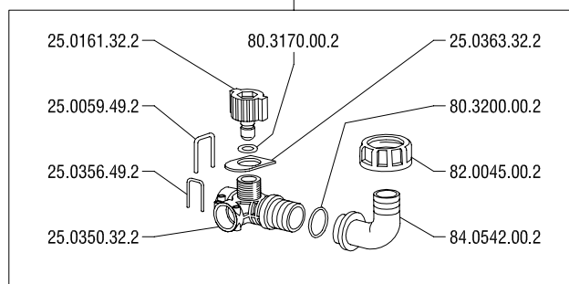
Terminal by-pass kit
